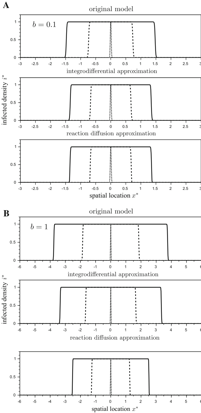
Fig. 2 The solutions of the original model (4), its integrodifferential approximation (8), and its lower-order reaction-diffusion approximation (10), for t^* = 0 (dotted), t^* = 100 (dashed), and t^* = 200 (solid), with d = 10^{-2} , \epsilon = 10^{-5} , a = 10^{-2} , and b = 0.1 (A), or b = 1 (B). This figure shows that the disease spreads as a travelling wave, and that the approximations are better for low b values
