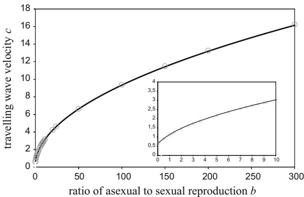
Fig. 6 Travelling wave velocity \hat{c} as a function of the ratio of asexual to sexual spore production b , from the reaction-diffusion approximation (10). Calculated points (Sect. 3.2) are represented by open circles. The curve corresponds to \hat{c} = .612\sqrt{2.317b + 1}
