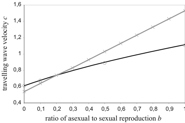
Fig. 3 Travelling wave velocity c^* as a function of the ratio of asexual to sexual spore production b . The black curve corresponds to the reaction-diffusion approximation (10), and the grey curve corresponds to the integrodifferential approximation (8), which is numerically very close to the original model (4) for \epsilon = 10^{-5} . Circles and crosses represent numerically calculated points for d = 10^{-2} , and a = 10^{-2}
