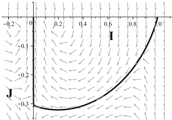
Fig. 4 Phase plane solution for \hat{c} \approx 0.612 in the strictly sexual case ( b = 0 )
