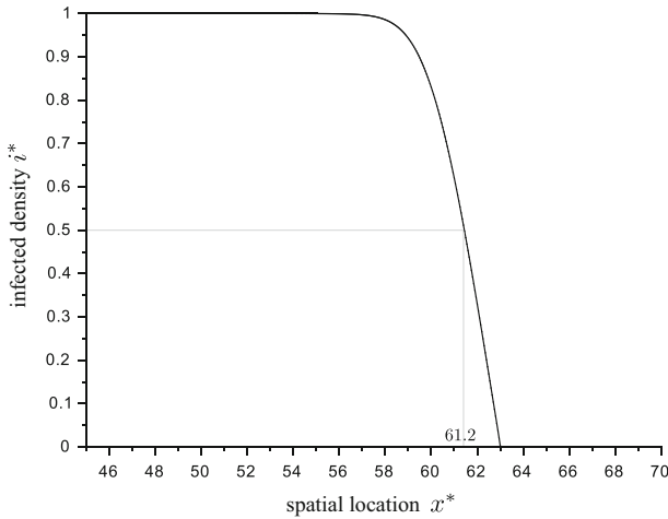
Fig. 5 The solid line corresponds to Eq. (10) numerical solution at t^* = 100 in the strictly sexual case ( b = 0 ), with initial conditions i^*(x^*) = 1 for -.01 \leq x^* \leq .01 , i^*(x) = 0 elsewhere. The wave front is at x^* \approx 61.2 , which confirms the mathematical analysis ( c^* = d\hat{c}/a = 0.612 with d = 10^{-2} , and a = 10^{-2} )
